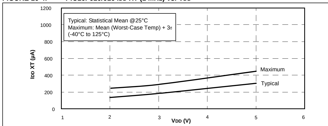
FIGURE 16-4: PIC16F610/616 I_{DD\ XT} (1 MHz) vs. V_{DD}
