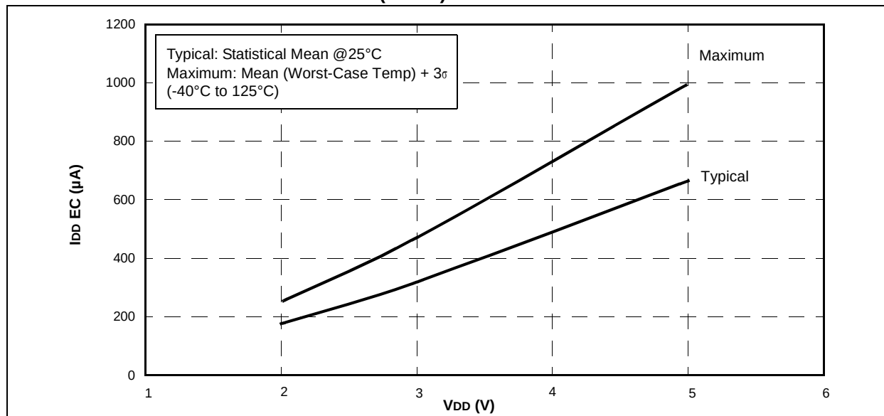
FIGURE 16-3: PIC16F610/616 I_{DD\ EC} (4 MHz) vs. V_{DD}
