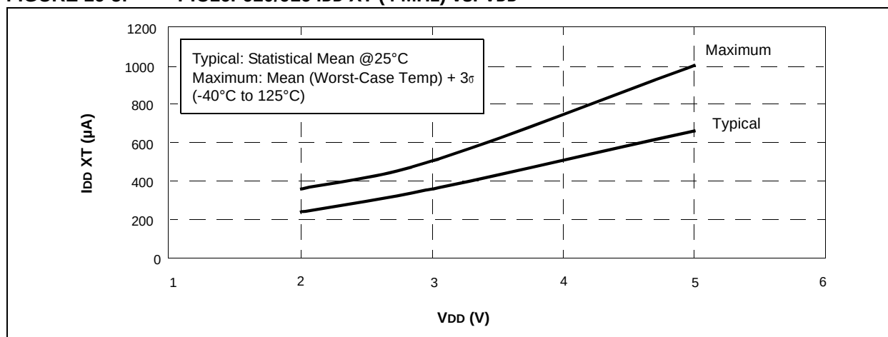
FIGURE 16-5: PIC16F610/616 I_{DD\ XT} (4 MHz) vs. V_{DD}
