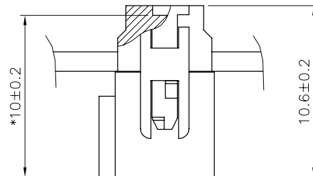
WITHOUT STRAIN RELIEF DUAL ENTRY COVER
