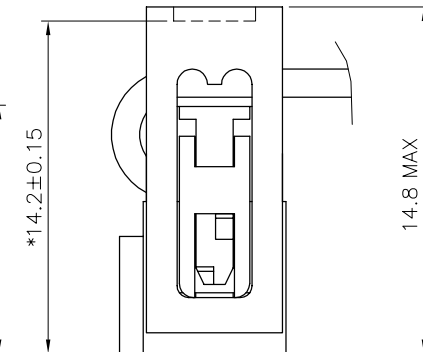
WITH LOW PROFILE STRAIN RELIEF
