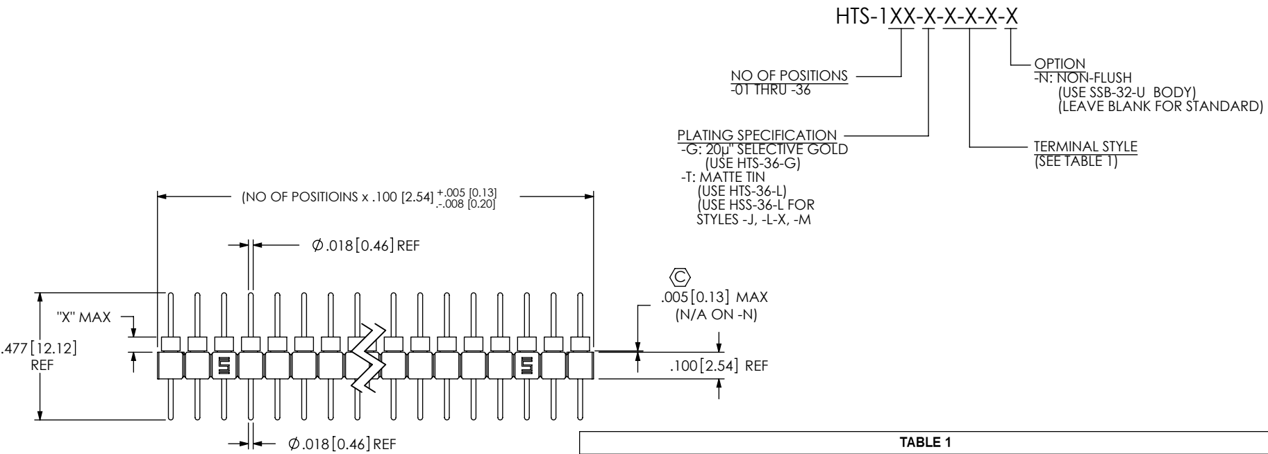
FIG 1 HTS-120-X-AA-T SHOWN
