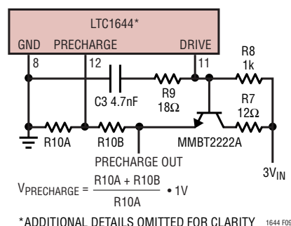
Figure 9. Precharge Voltage &gt;1V Application Circuit
