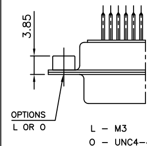
CLINCH NUT
