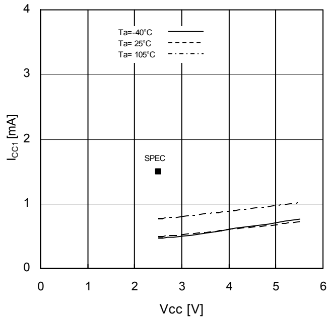
Figure 11. Supply Current (Write) vs Supply Voltage (fSCK=5MHz)
