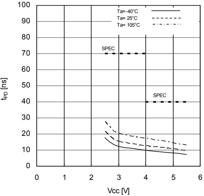
Figure 23. Data Output Delay Time vs Supply Voltage
