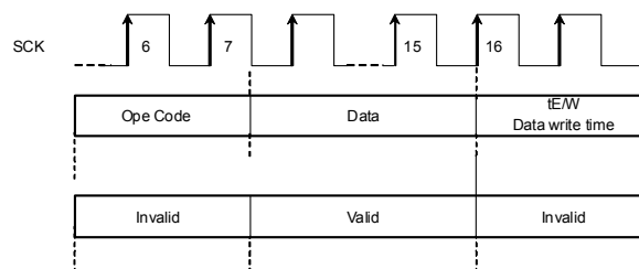
Figure 38. WPB valid timing (At inputting WRSR command)
