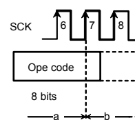
Figure 43. WREN/WRDI cancel valid timing
