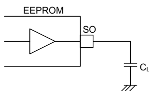
Figure 46. SO load capacity
