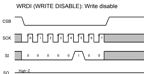
Figure 33. Write disable command
