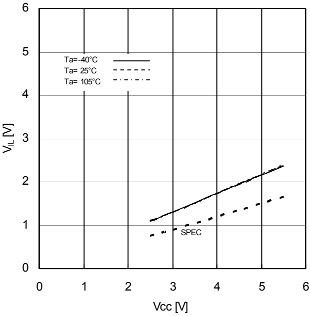
Figure 6. Input Low Voltage vs Supply Voltage (CSB,SCK,SI,HOLDB,WPB)
