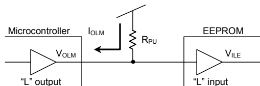
Figure 44. Pull up resistance
