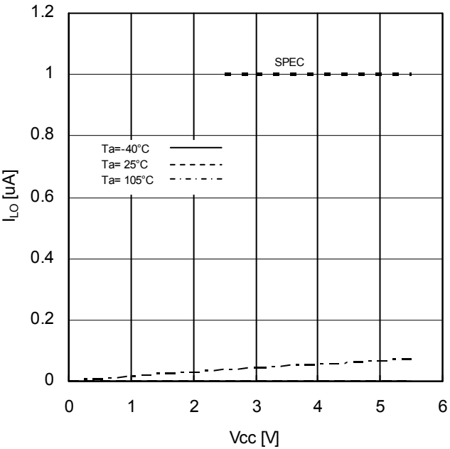
Figure 10. Output Leakage Current vs Supply Voltage (SO)
