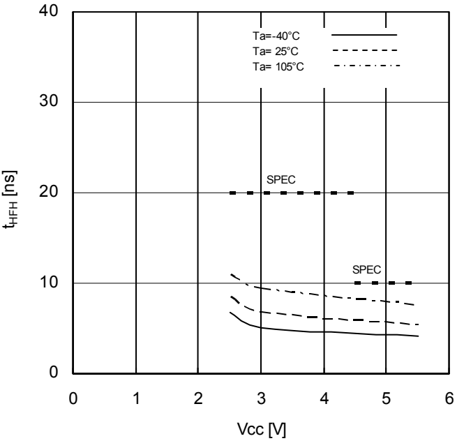
Figure 25. HOLDB Setting Hold Time vs Supply Voltage
