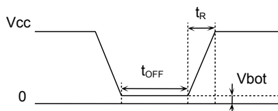
Figure 55. Rise waveform
