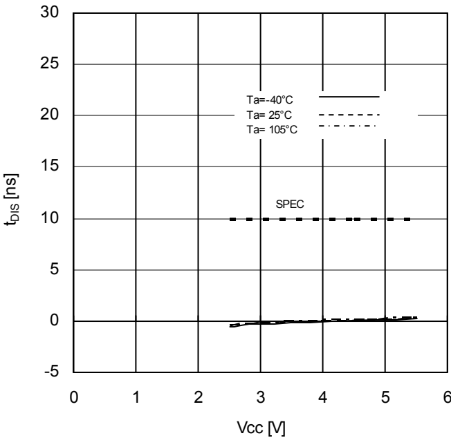
Figure 21. SI Setup Time vs Supply Voltage
