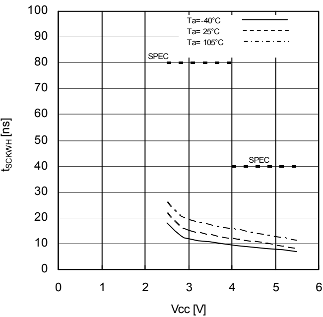
Figure 16. SCK High Time vs Supply Voltage
