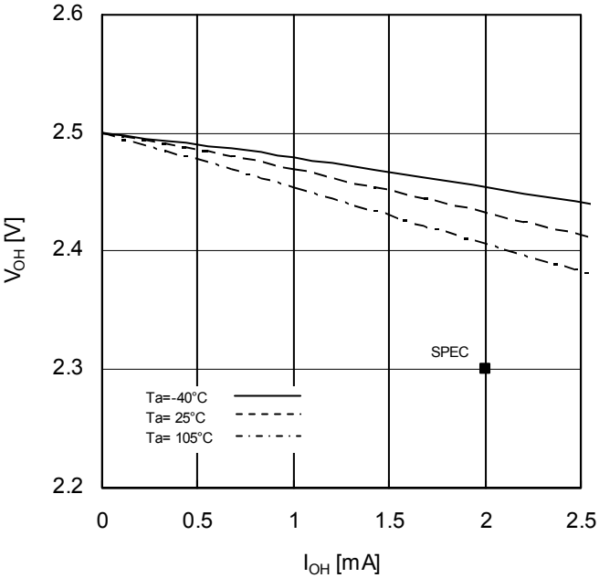
Figure 8. Output High Voltage vs Output Current (Vcc=2.5V)
