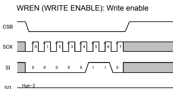
Figure 32. Write enable command
