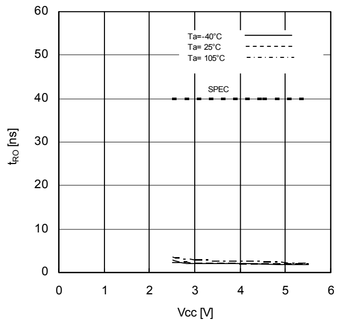
Figure 29. OUTPUT Rise Time vs Supply Voltage
