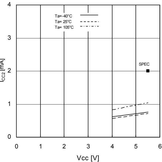
Figure 12. Supply Current (Write) vs Supply Voltage (fSCK=10MHz)
