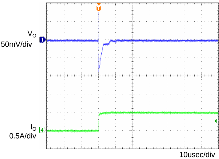
Fig.3 Transient Response (0 \rightarrow 0.5A) Co=1 \mu F, Ta=-40°C
