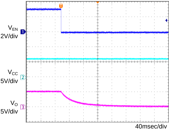
Fig.19 OFF sequence 2 Co=1μF, Ta=25°C
