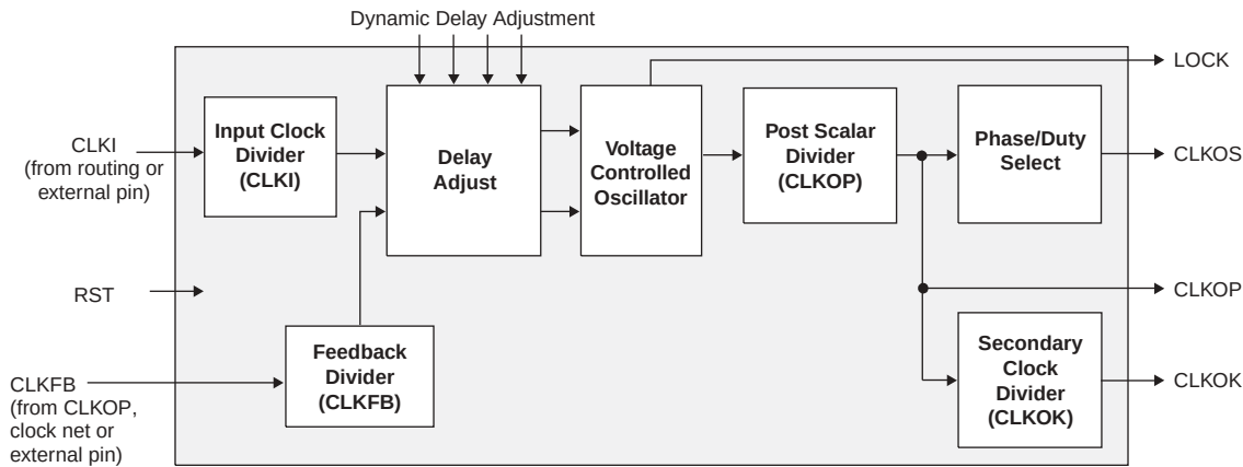
Figure 2-11. PLL Diagram
