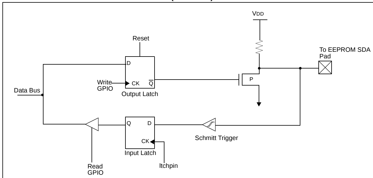
FIGURE 6-1: BLOCK DIAGRAM OF GPIO6 (SDA LINE)
