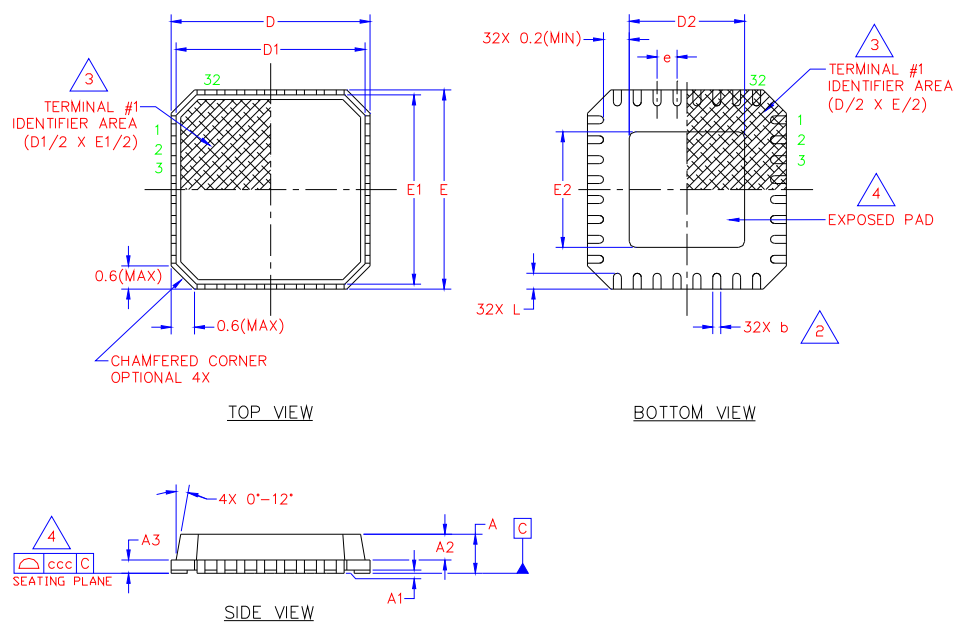
Figure 9 USB3300-EZK 32 Pin QFN Package Outline, 5 x 5 x 0.9 mm Body (Lead-Free)
