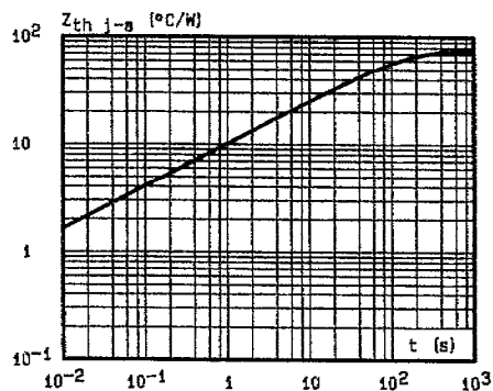
Fig.3 - Transient thermal impedance junction-ambient for mounting n°2 versus pulse duration ( L = 10 \text{ mm} ).
