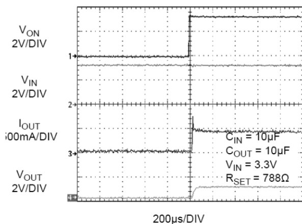
Figure 23. Current Limit Response Time (Output is Loaded by 2.2\ \Omega , C_{OUT}=10\ \mu\text{F} )
