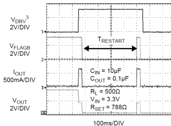
Figure 26. t_{RESTART} vs. Response (3)
