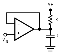
Figure 53. Compensating for Large Capacitive Loads with a Pull Up Resistor
