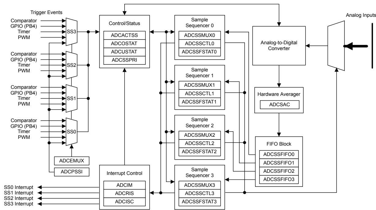
Figure 11-1. ADC Module Block Diagram
