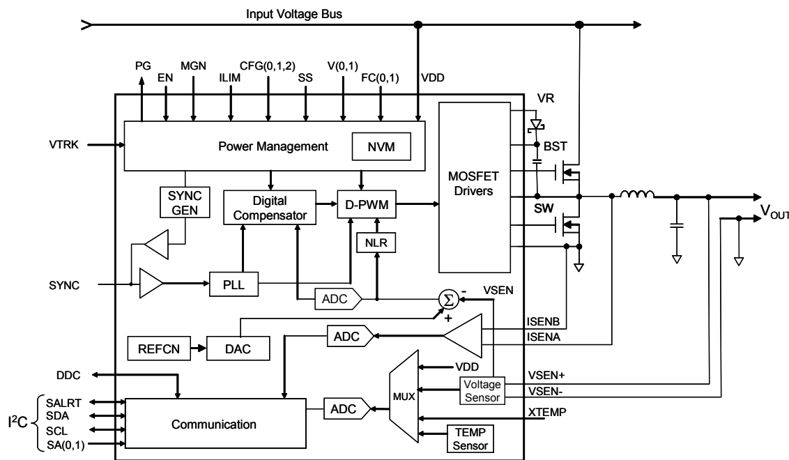
FIGURE 4. ZL2008 Block Diagram
