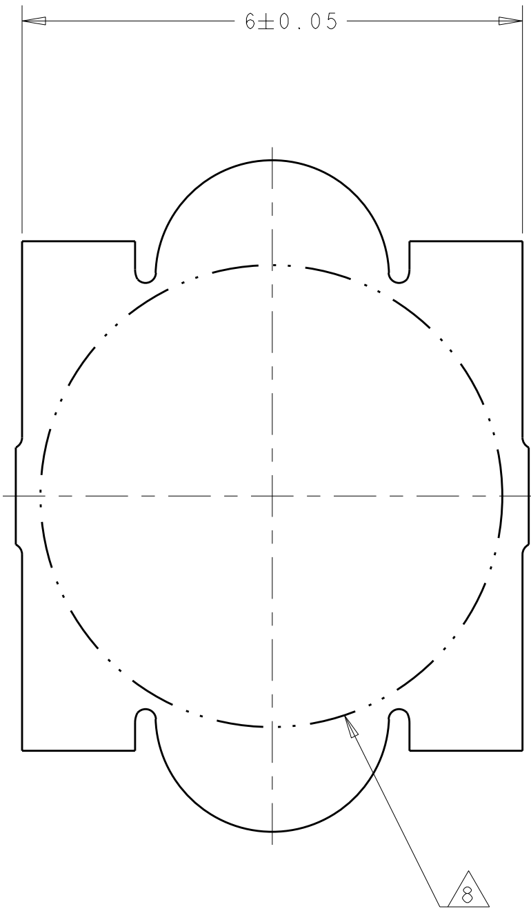
VACUUM COVER
