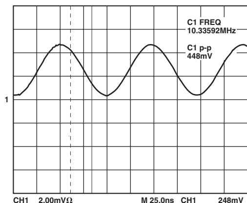
Figure 14. DAC Output
