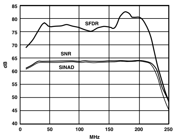
TPC 18. SNR, and SINAD, SFDR vs. Clock Rate; ( A_{IN} = 10.3 MHz, @ -0.5 dBFS), LVDS Mode, Full Scale = 1.536 V, -210 Grade
