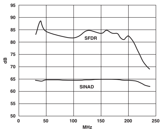
TPC 17. SINAD and SFDR vs. Clock Rate ( A_{IN} = 10.3 MHz @ -0.5 dBFS, LVDS Mode), -170 Grade
