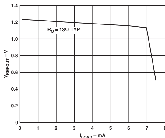
TPC 23. V_{REFOUT} vs. I_{LOAD}
