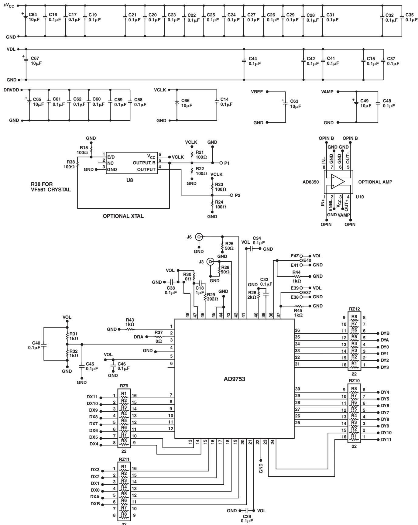
Figure 18b. Evaluation Board Schematic (continued)
