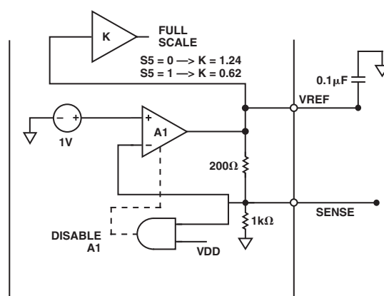
Figure 6. VREF, SENSE I/O
