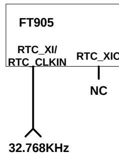
Figure 6-4 External 32.768 KHz clock input
