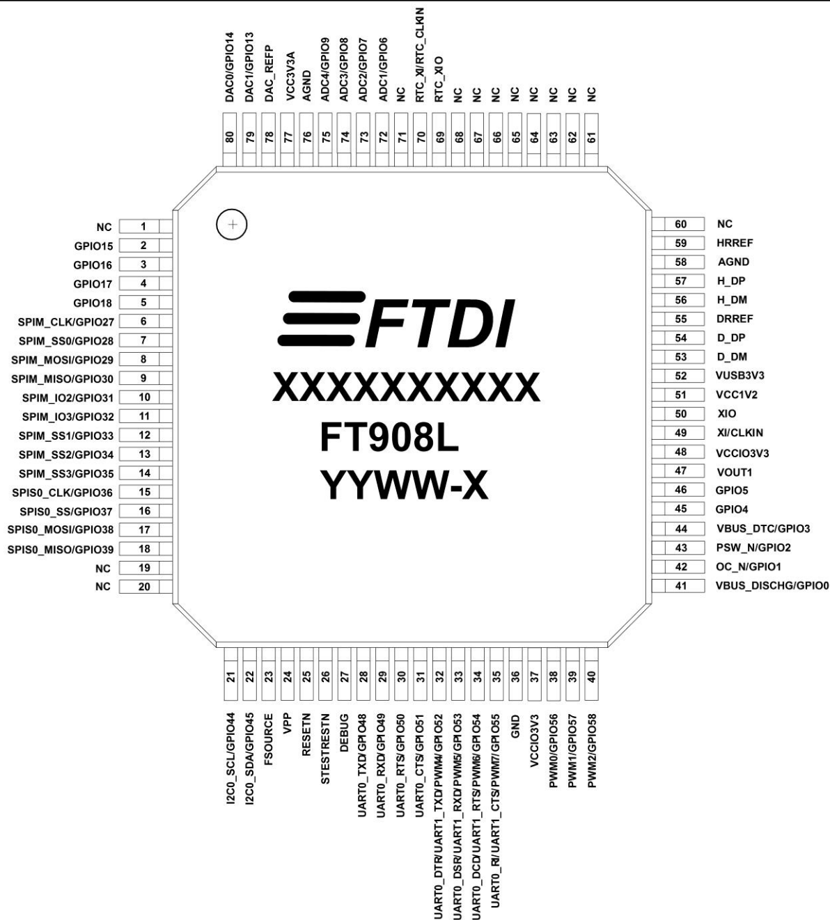
Figure 3-8 Pin Configuration FT908L (top-down view)
