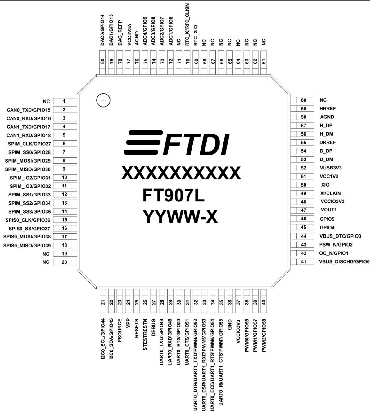
Figure 3-7 Pin Configuration FT907L (top-down view)
