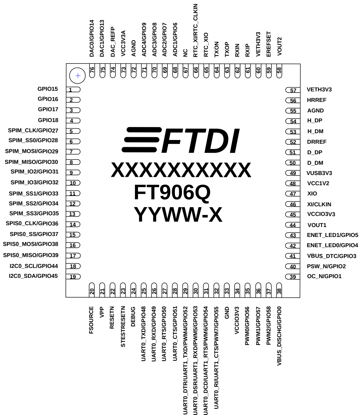
Figure 3-2 Pin Configuration FT906Q (top-down view)
