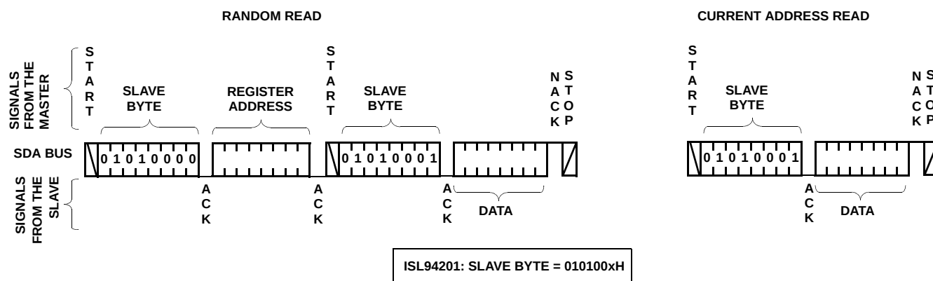
FIGURE 10. READ SEQUENCE
