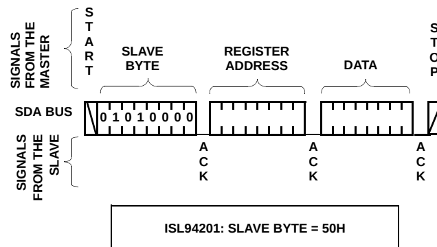
FIGURE 9. WRITE SEQUENCE
