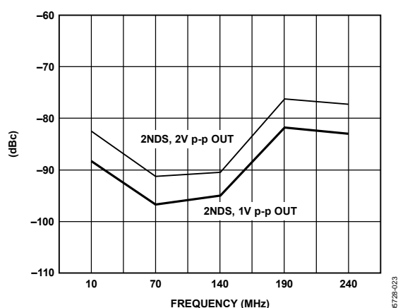
Figure 28. Single-Ended, Second-Order Harmonic Distortion, 1 kΩ Load
