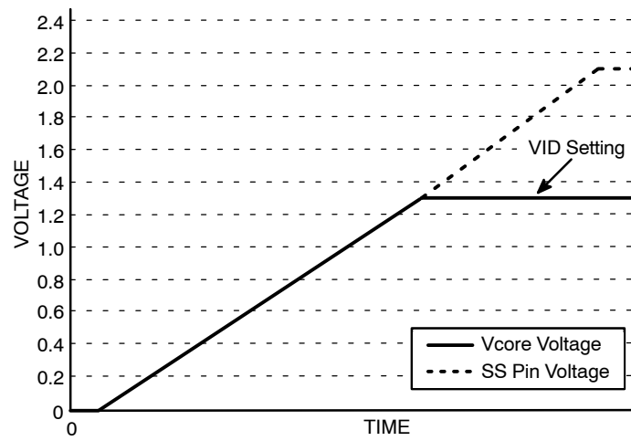
Figure 8. Typical VR10 Soft-Start Sequence to V_{core} = 1.3\text{ V}
