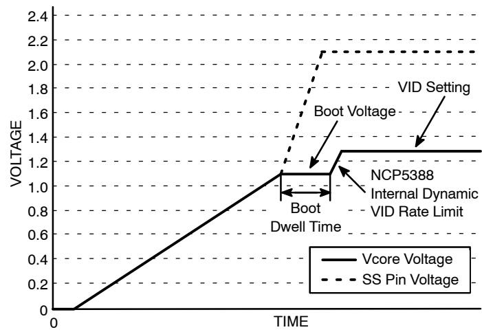
Figure 9. Typical VR11 Soft-Start Sequence to V_{core} = 1.3\text{ V}
