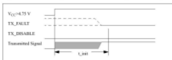
Power on initialization of GBIC, TX_DISABLE negated
