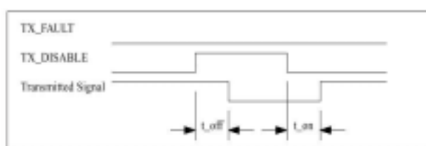
Management of GBIC during normal operation, TX_DISABLE implemented
