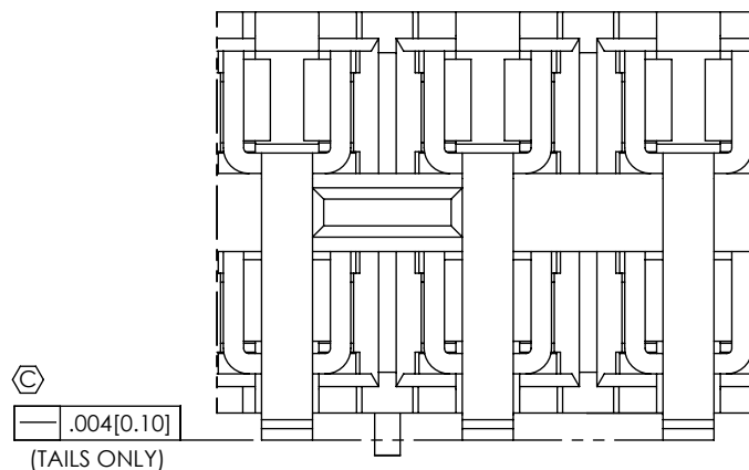
DETAIL 'D' SCALE 12:1
