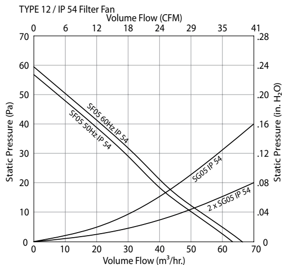
SF05 39 CFM (66 m³/hr.) Side-Mount Filter Fan Performance Curve
