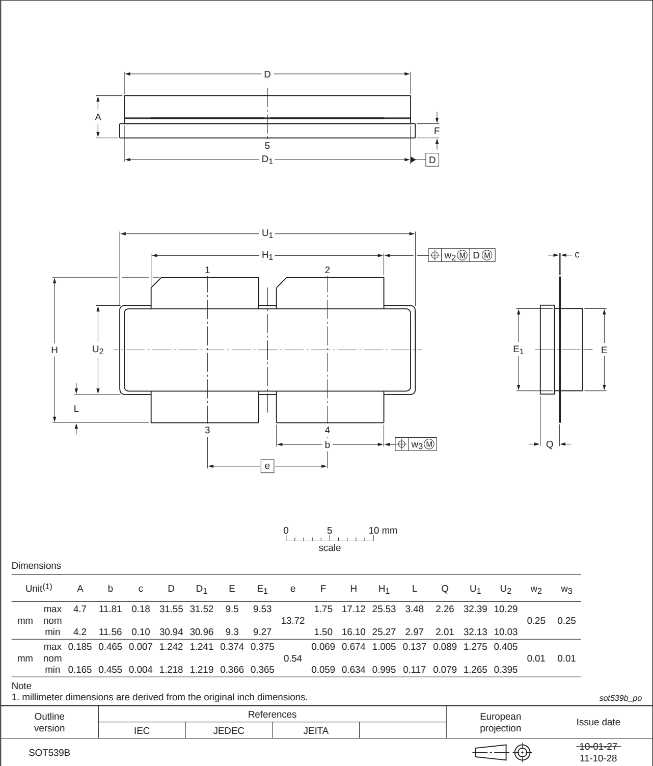
Earless flanged balanced LDMOST ceramic package; 4 leads SOT539B
