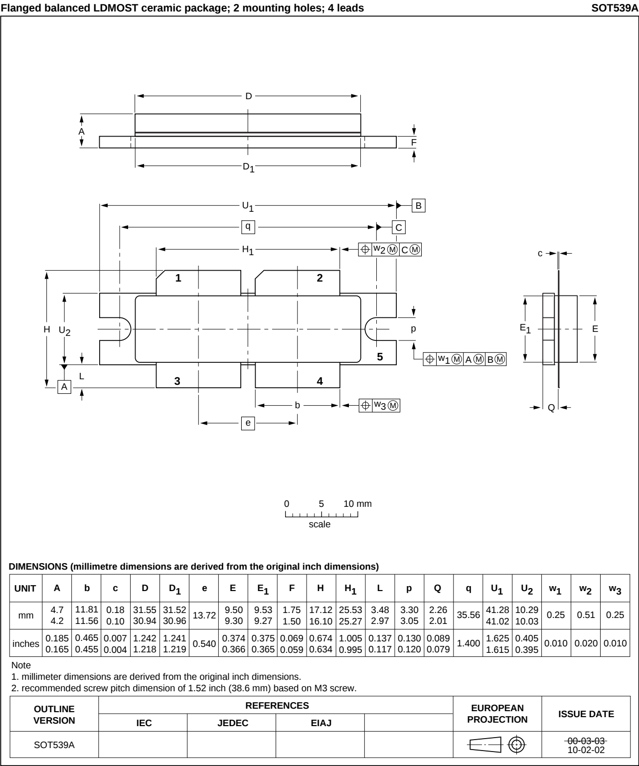
Fig 1. Package outline SOT539A
