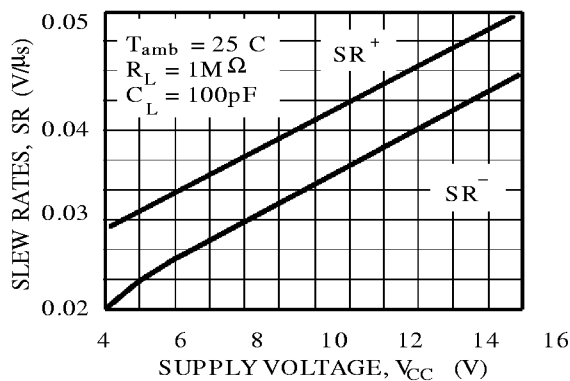
Figure 9 : Slew Rates versus Supply Voltage
