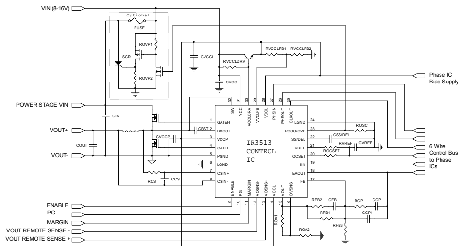
Figure 1 - IR3513 Application Circuit
