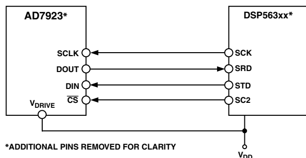
Figure 20. Interfacing to the DSP563xx
