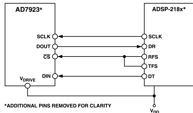
Figure 19. Interfacing to the ADSP-218x
