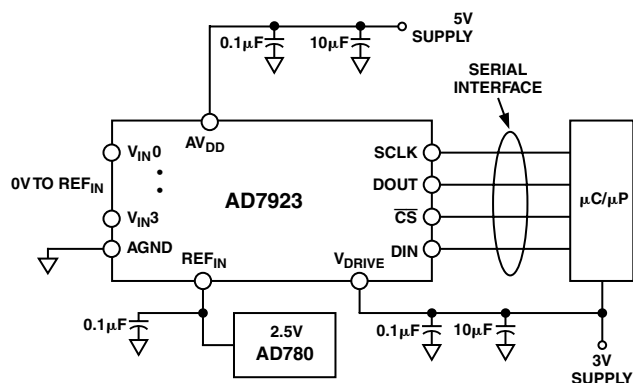
Figure 10. Typical Connection Diagram
