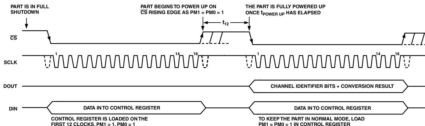
Figure 12. Full Shutdown Mode Operation
