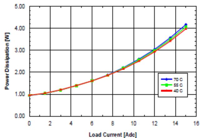
Fig. 1.2V.8: Power dissipation vs. load current and ambient temperature for SQ48T/S15012 converter mounted vertically with V_{in} = 48\text{V} and air flowing from pin 3 to pin 1 at a rate of 200LFM (1.0 m/s).
