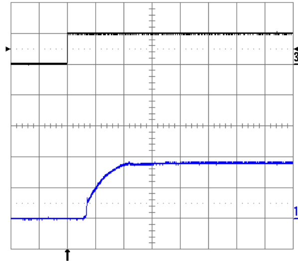
Fig. 1.8V.10: Turn-on transient at full rated load current (resistive) plus 10,000 \mu F at V_{in} = 48V , triggered via ON/OFF pin. Top trace: ON/OFF signal (5V/div.). Bottom trace: output voltage (1V/div.). Time scale: 2ms/div.
