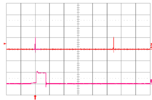
Fig. 2.0V.16: Input reflected ripple current, i_s (10 mA/div.), measured through 10\mu\text{H} at the source at full rated full rated load current and V_{in} = 48\text{V} . Refer to Fig. 2.0V.14 for test setup. Time scale: 1\mu\text{s}/\text{div} .
