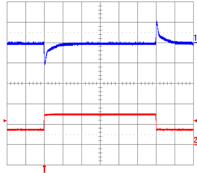
Fig. 1.8V.12: Output voltage response to load current step-change (3.75 A – 7.5 A – 3.75 A) at V_{in} = 48V . Top trace: output voltage (100 mV/div.). Bottom trace: load current (5A/div.). Current slew rate: 5 A/ \mu s . C_o = 450\mu F tantalum + 1 \mu F ceramic. Time scale: 0.2 ms/div.
