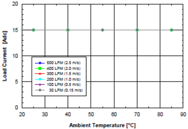
Figure 1.0V.4 Available load current vs. ambient air temperature and airflow rates for SQ48S15010 converter with D height pins mounted horizontally with V_{in} = 48V , air flowing from pin 3 to pin 1, and maximum FET temperature \leq 120^{\circ}C .
