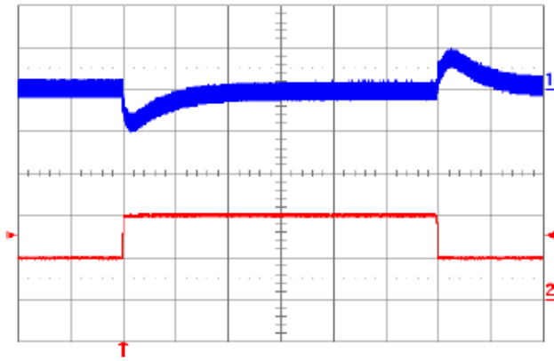
Fig. 12V.9: Output voltage response to load current step-change (1A – 2A – 1A) at V_{in} = 48V . Top trace: output voltage (200mV/div.). Bottom trace: load current (1A/div.). Current slew rate: 0.1A/ \mu s. C_o = 1\mu F ceramic. Time scale: 0.5 ms/div.
