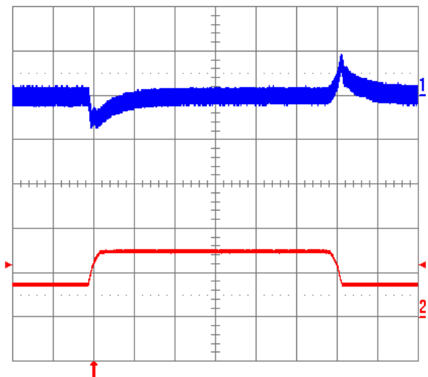
Fig. 3.3V.11: Output voltage response to load current step-change (3.75 A – 7.5 A – 3.75 A) at V_{in} = 48V . Top trace: output voltage (100mV/div.). Bottom trace: load current (5A/div.). Current slew rate: 0.1A/ \mu s . C_o = 1\mu F ceramic. Time scale: 0.2 ms/div.
