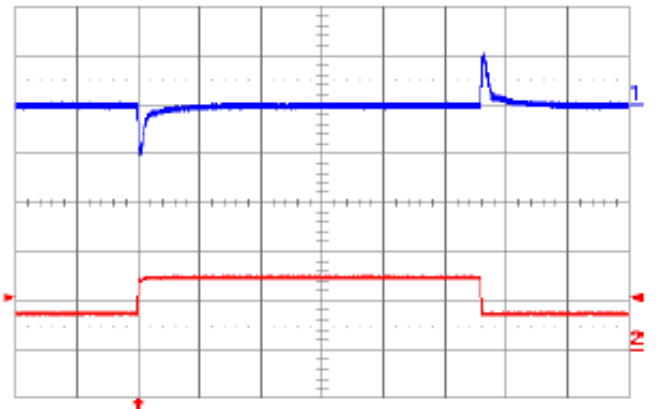
Fig. 1.0V.12: Output voltage response to load current step-change (3.75 A - 7.5 A - 3.75 A) at V_{in} = 48V . Top trace: output voltage (100 mV/div.). Bottom trace: load current (5A/div.). Current slew rate: 5 A/ \mu s . C_o = 450\mu F tantalum + 1 \mu F ceramic. Time scale: 0.2 ms/div.
