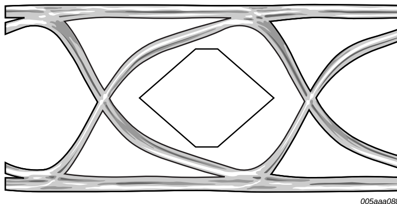
Fig 3. Eye diagram at 1 V receiver common-mode
