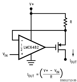
FIGURE 21. Large Compliance Range Current Source
