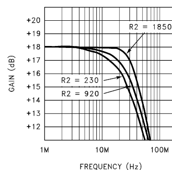
FIGURE 4. FREQUENCY RESPONSE vs RESISTOR R2 (GAIN = 8)
