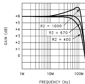
FIGURE 2. FREQUENCY RESPONSE vs RESISTOR R2 (GAIN = 2)
