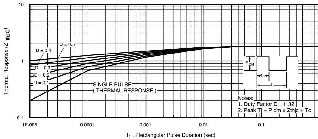
Fig. 4 - Max. Thermal Impedance Z_{thJC} Characteristics
