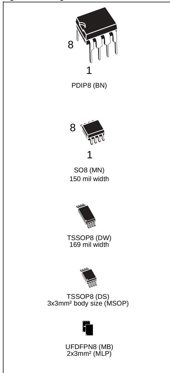
Figure 1. Packages
