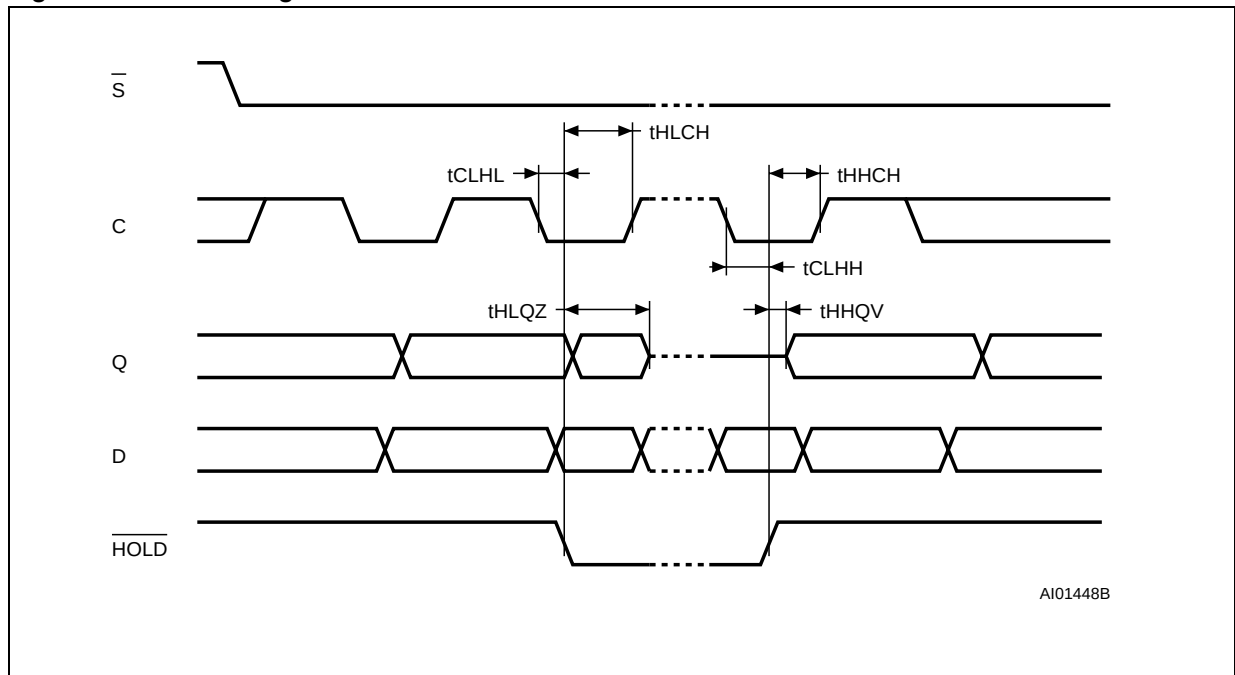
Figure 16. Hold Timing
