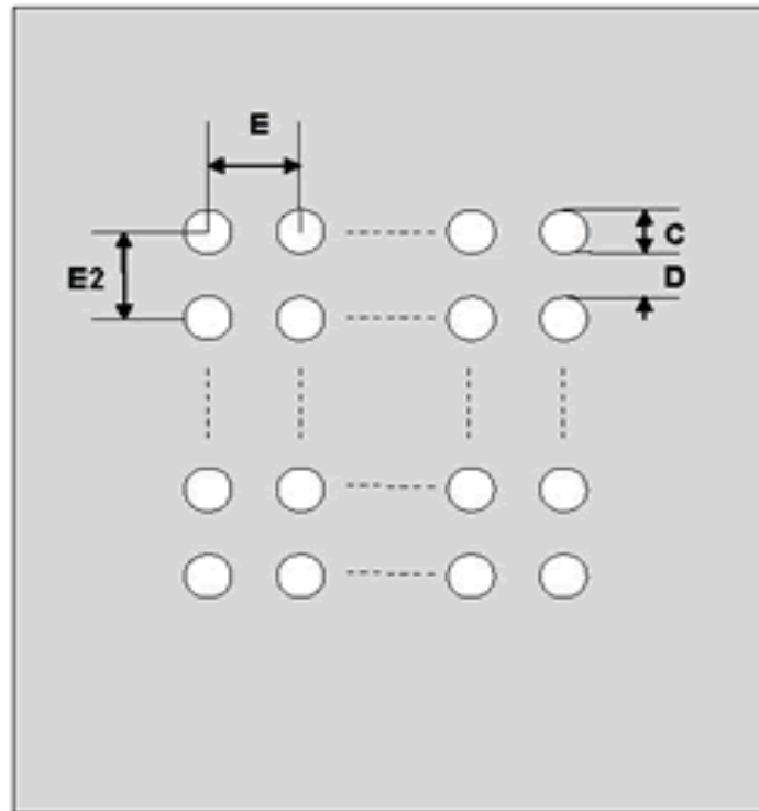
Top View (SMT Footprint)
