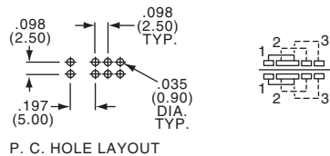
P. C. HOLE LAYOUT
