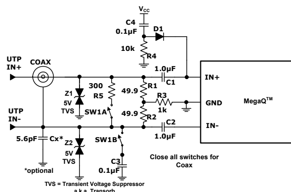
FIGURE 47. APPLICATION CIRCUIT FOR UTP/COAX CABLE
