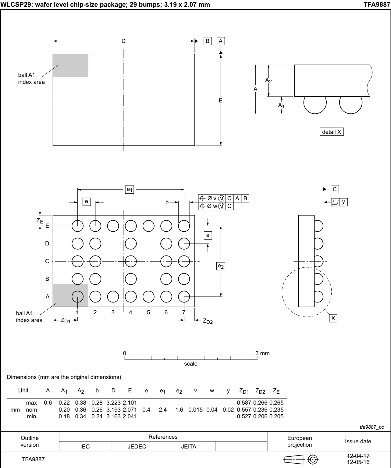
Fig 5. Package outline TFA9887 (WLCSP29)
