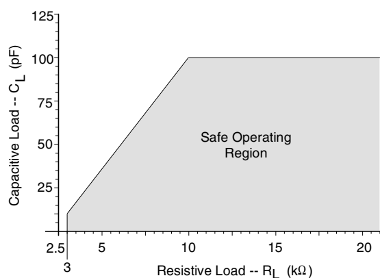
Figure 2. Maximum Loading
