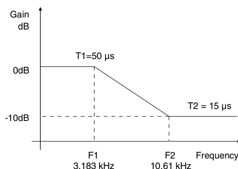
Figure 20. De-Emphasis Curve
