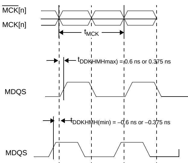
Figure 12. MCK to MDQS Timing
