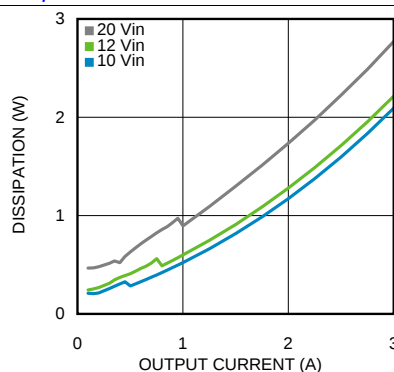
Figure 20. Dissipation 6-V Output at 85°C Ambient
