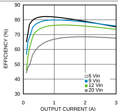
Figure 25. Efficiency 2.5-V Output at 85°C Ambient
