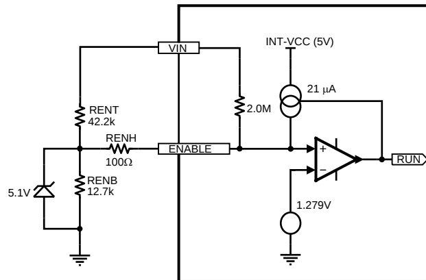
Figure 47. Enable Input Detail
