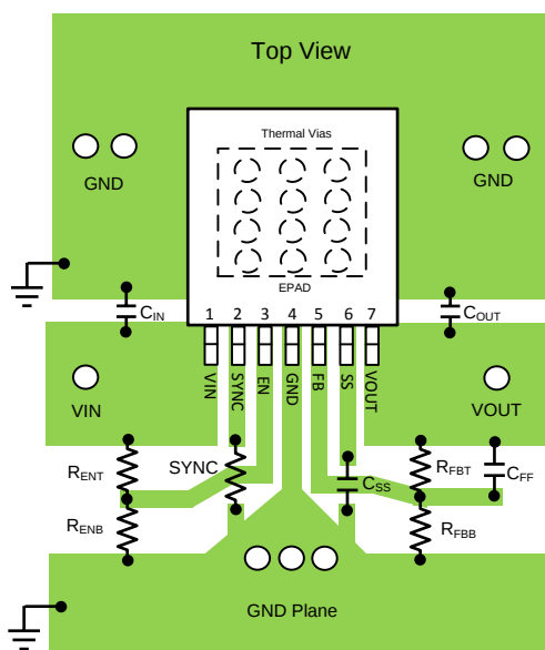
Figure 53. PCB Layout Guide
