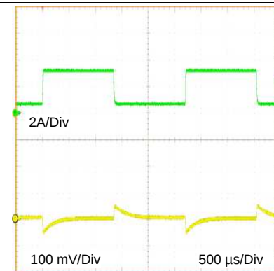
Figure 40. Output Ripple
