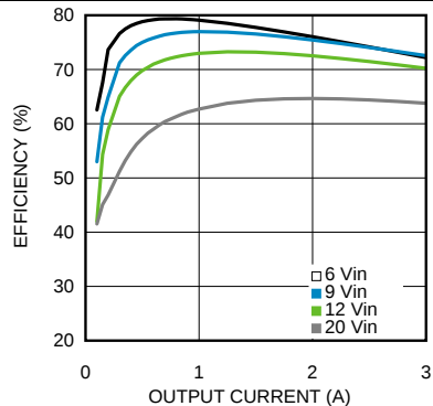
Figure 27. Efficiency 1.8-V Output at 85°C Ambient
