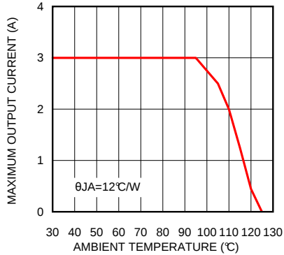
Figure 37. Thermal Derating
