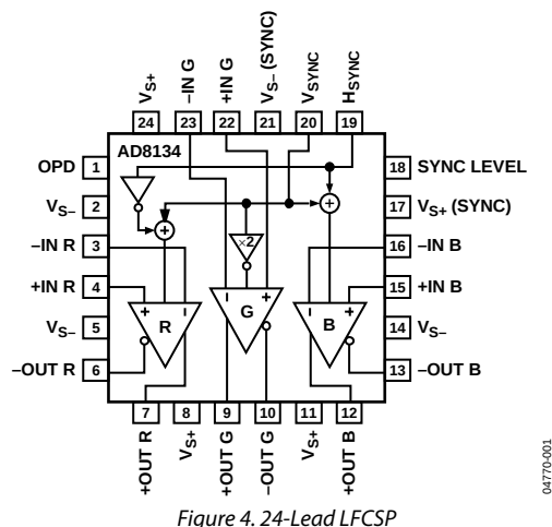
Figure 4. 24-Lead LFCSP
