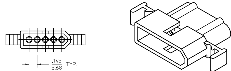
PLUG HOUSING SHOWN WITH STANDARD EARS
