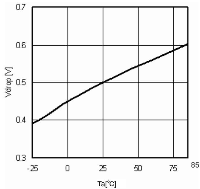
Fig.18 Minimum dropout Voltage 1 ( V_{CC}=5\text{V} , I_O=-1.0\text{A} )
