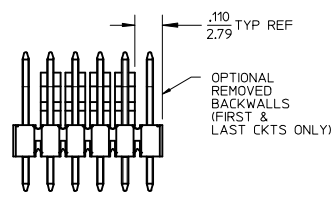
REMOVED BACKWALLS OPTION SEE NOTE 11
