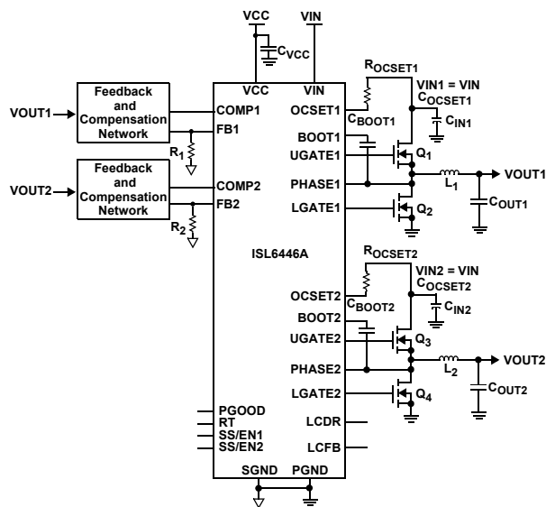
FIGURE 1. TYPICAL APPLICATION
