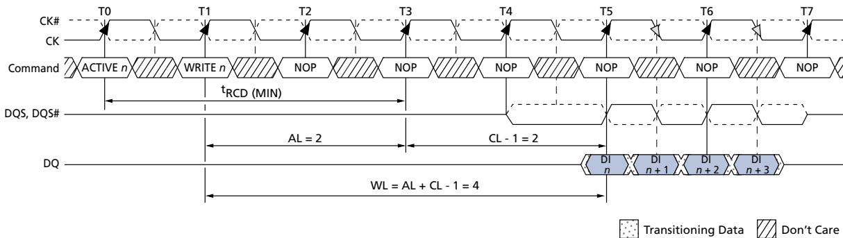
Figure 42: WRITE Latency
