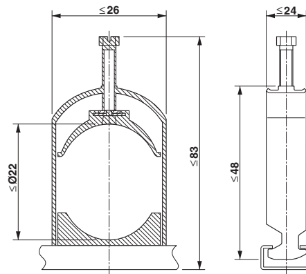
Dimensioned drawing
