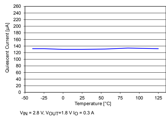
Figure 9. Quiescent current vs. temperature ( I_{OUT} = 200 \text{ mA} )
