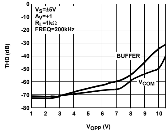
FIGURE 18. TOTAL HARMONIC DISTORTION vs OUTPUT VOLTAGE
